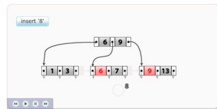
Fig. 2. Snapshots on B+ tree Insertion Animation in Database implementation course, one of animation mentioned by students.
