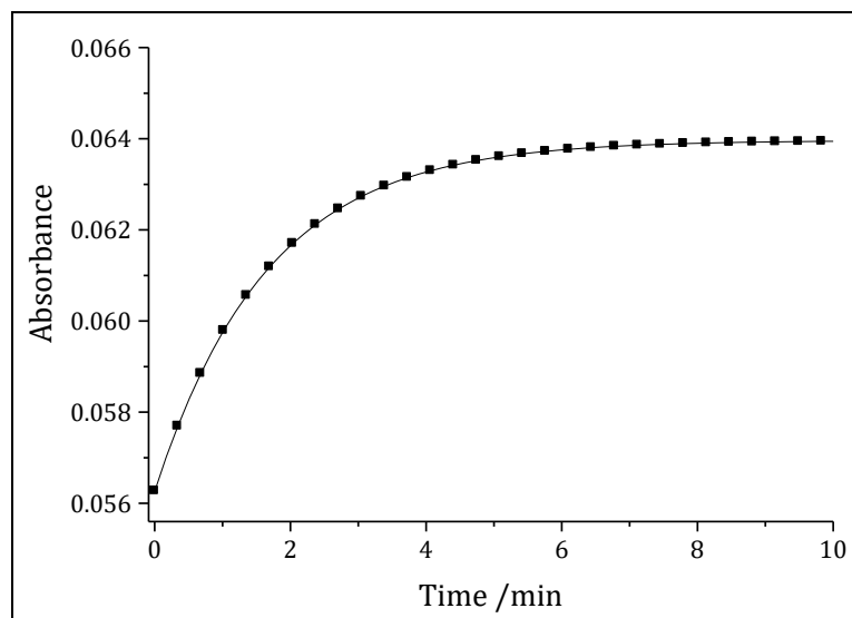
Figure 1: Stopped-Flow kinetic trace of Pt3 (0.2 mM) with 6 mM thiourea at 298 K in methanol, I = 0.1 M (NaClO 4 /LiCl)
