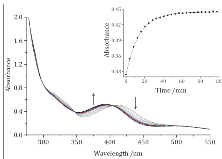
Figure 2: UV-Vis spectra recorded as a function of time for the reaction between Pt2 and 6 mM of thiourea at 25 °C in methanol, I = 0.1 M (NaClO 4 /LiCl). Inset is the kinetic trace obtained at 375 nm.
