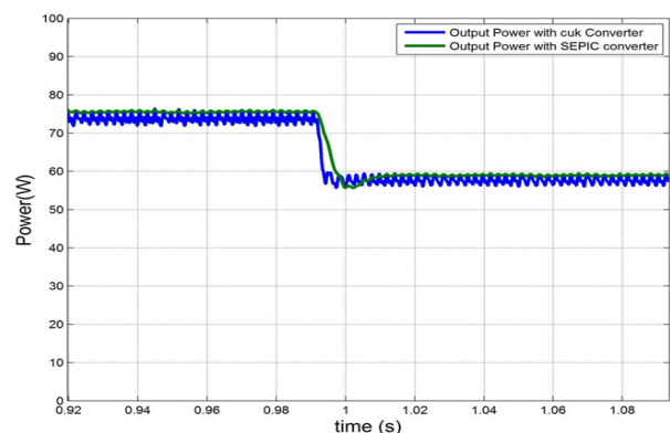
Fig. 10 Expanded time scale waveform of power for a step change of temperature from 25°C to 50°C and constant irradiance of 1 kW/m 2
