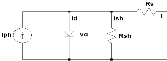
Fig. 1 Schematic diagram of single diode solar cell
