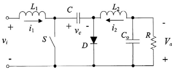
Fig. 4 Circuit diagram of Ćuk converter
