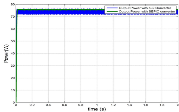
Fig. 7 Power at constant temperature of 25°C and constant irradiance of 1 kW/m²
